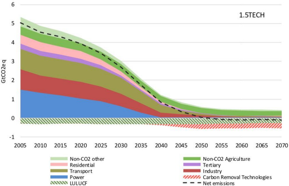
Figure 90: Two ways to reach net zero GHG emissions - reduction pathways for 1.5TECH (above) and 1.5LIFE scenario (below) with enhanced LULUCF sink 451
